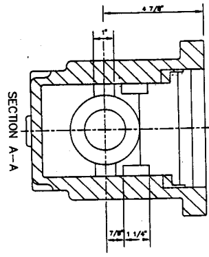
INTERNAL DIMENSIONS
