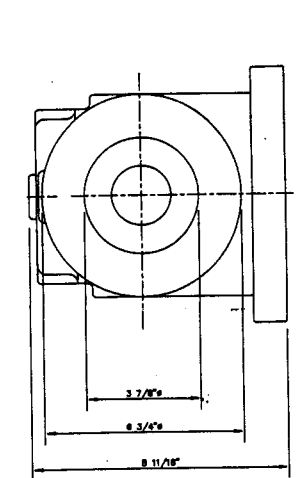
EXTERNAL DIMENSIONS
