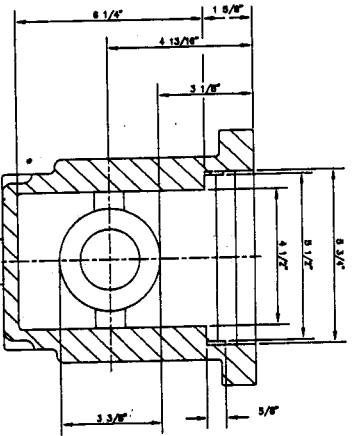
INTERNAL DIMENSIONS
