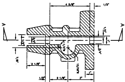
CAVITY DIMENSIONS
