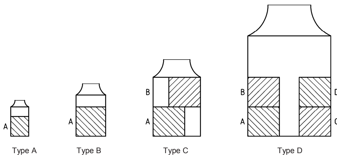
Figure G.2 — Sectioning procedure for cast-on samples Type A, Type B, Type C and Type D (see Figure 4)
