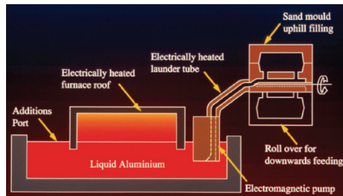
Fig. 11 The Cosworth counter-gravity casting process [48] .
