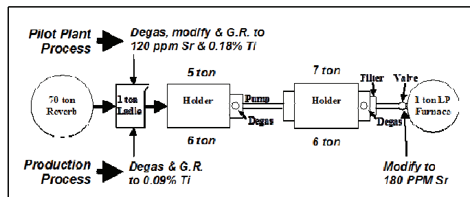
Fig. 8 Degassing locations used in both pilot plant and production plant at Nemak [44] .
