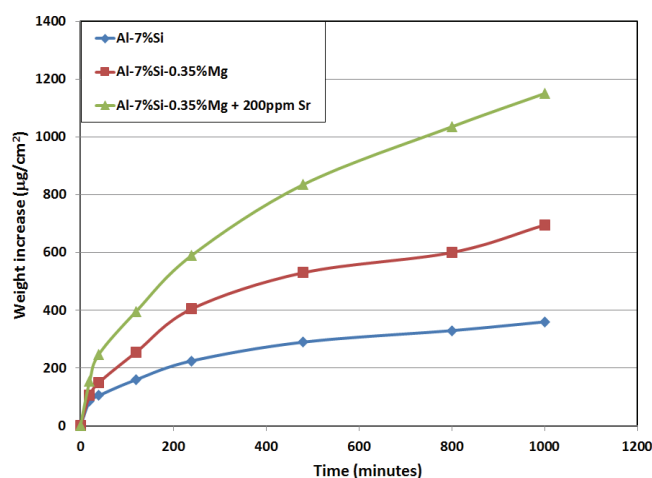
Fig. 4 Thermogravimetric analysis of oxidation rate of aluminum alloy (Al-7%Si) with or without Mg and Sr addition at 730^\circ\text{C} .
