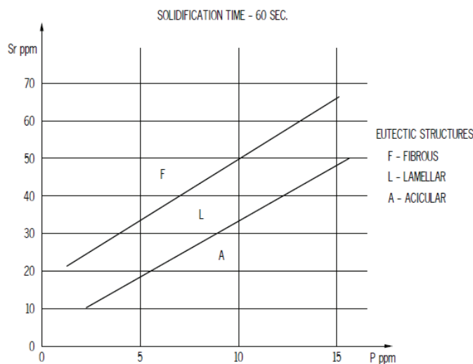
Fig. 3 Sr and P interaction in Al-7%Si alloy [27] .
