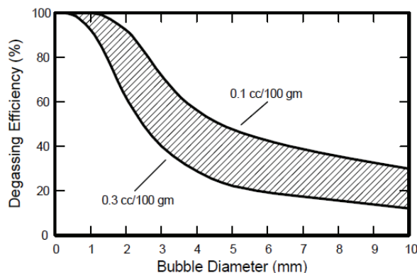
Fig. 6 Calculated degassing efficiency as a function of bubble size [40] .
