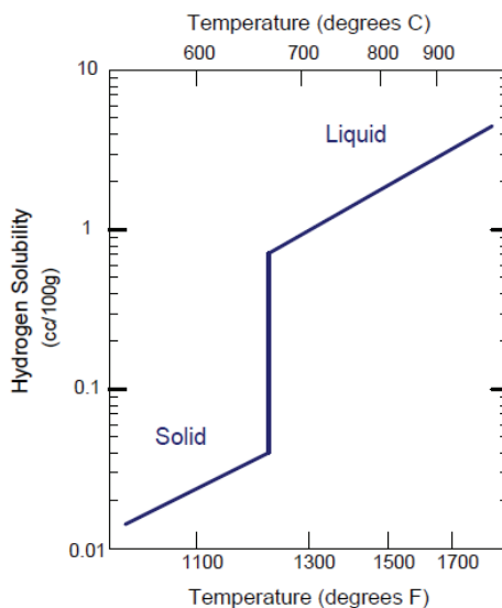
Fig. 5 Hydrogen solubility in pure aluminum [40] .
