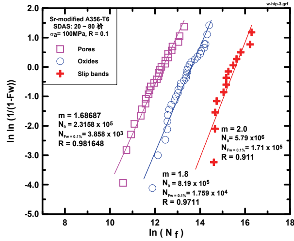
Fig. 1 Two-parameter Weibull plot for fatigue life of a Sr-modified A356 casting alloy sorted by the type of crack origin (pore, oxides, or slip bands) observed on the fracture [1, 13] .
