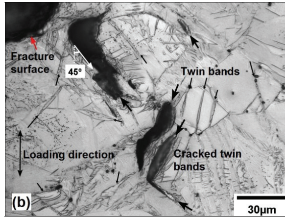
Fig. 2 SEM image showing crack initiation from the twin bands in the NZ30K1-T4 Mg alloy [24] .
