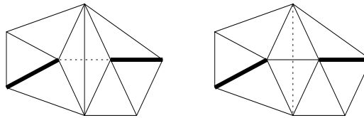
Figure 29: Edge swapping to give a constrained Delaunay triangulation
