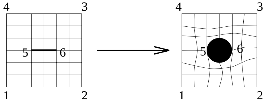
Figure 13: H type grid
