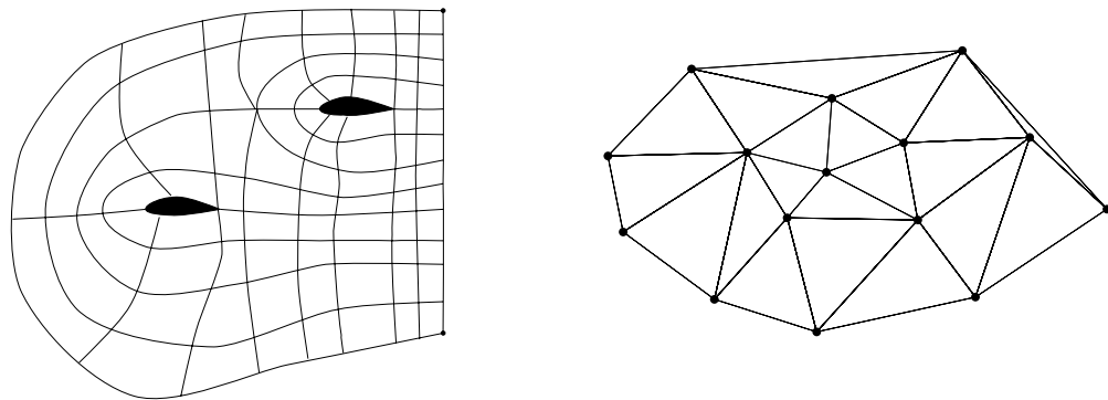
Figure 1: Structured mesh (left) and unstructured mesh (right).
