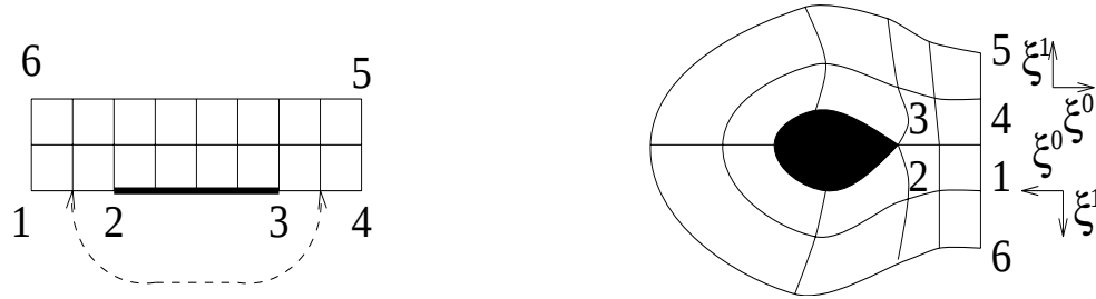
Figure 12: C type grid
