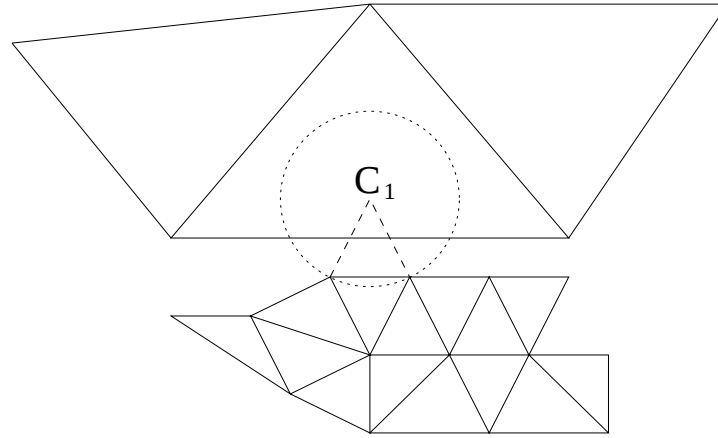
Figure 22: Element generation failure (side intersection) because of too small a value of search radius.
