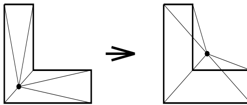
Figure 31: Failure of Laplacian smoothing
