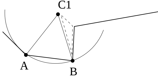
Figure 21: Poor choice of a new element will lead to distorted elements being produced later.
