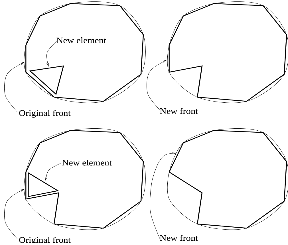
Figure 19: Advancing front
