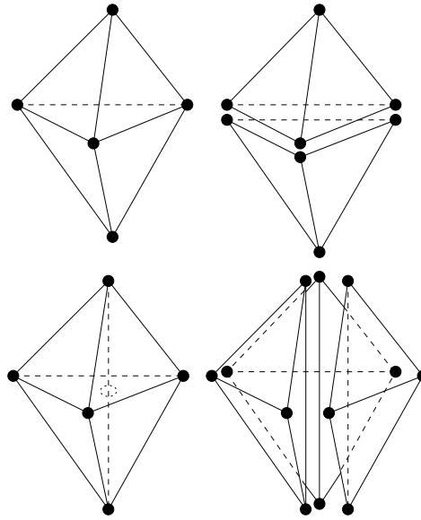
Figure 30: Face-edge swapping
