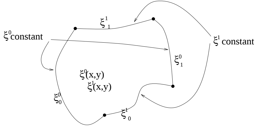
Figure 7: Elliptic grid generation boundaries
