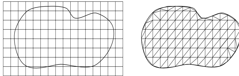
Figure 17: Overlaid grid, cropped, warped to boundary and split into triangles
