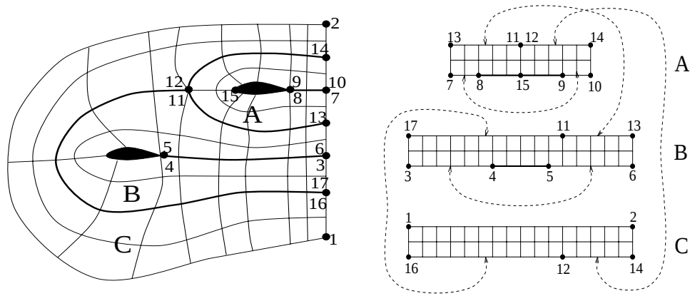
Figure 15: Example of multiblock: 3 C-type grids
