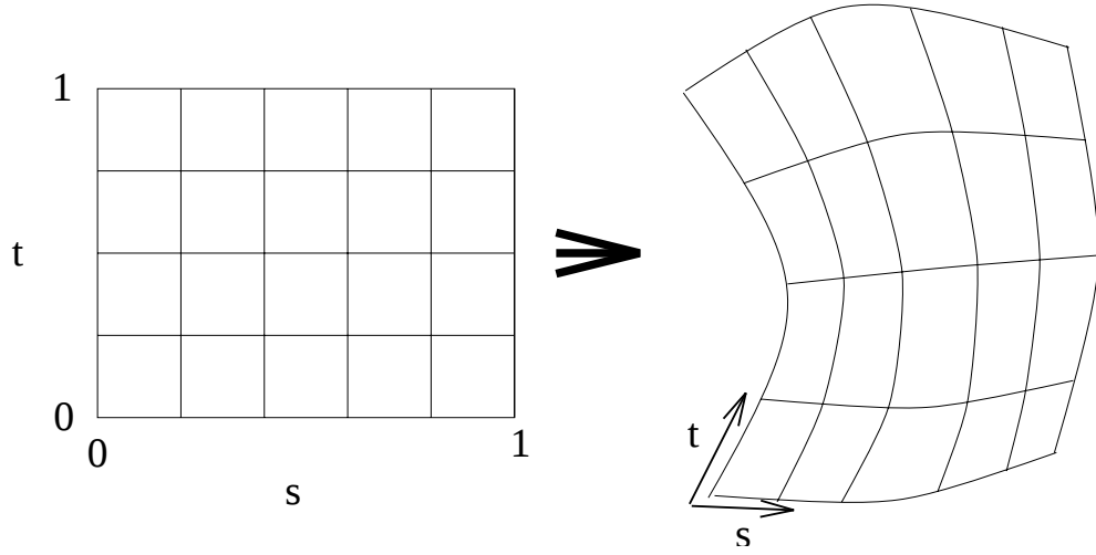
Figure 5: Transfinite interpolation
