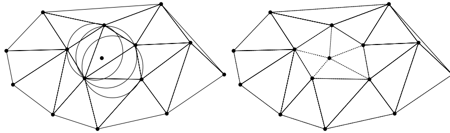
Figure 27: Bowyer-Watson triangulation: circumcircles that contain the new point, and the resulting triangulation
